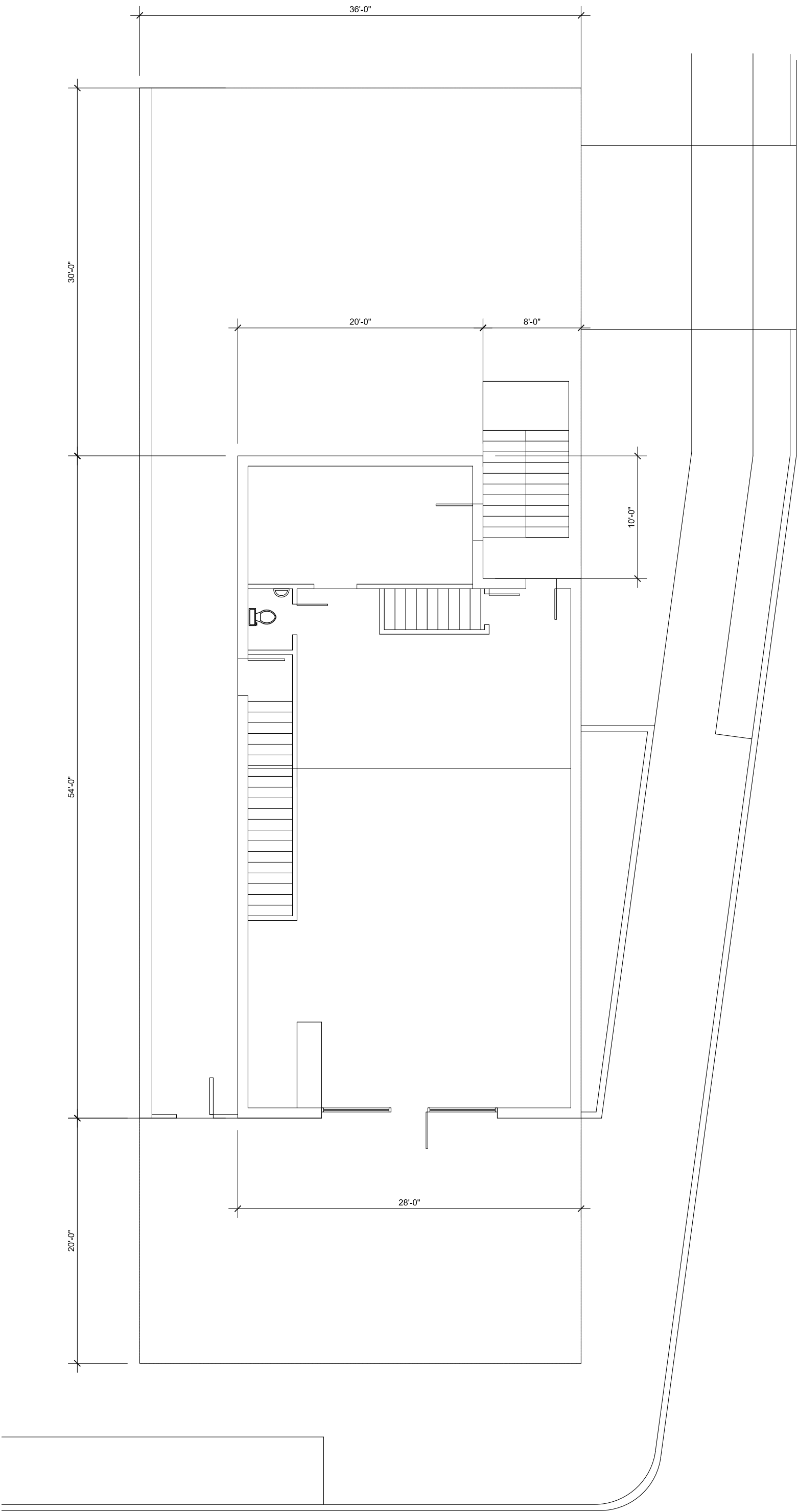
GROUND FLOOR PLAN SCALE: 1/4" = 1'-0"
